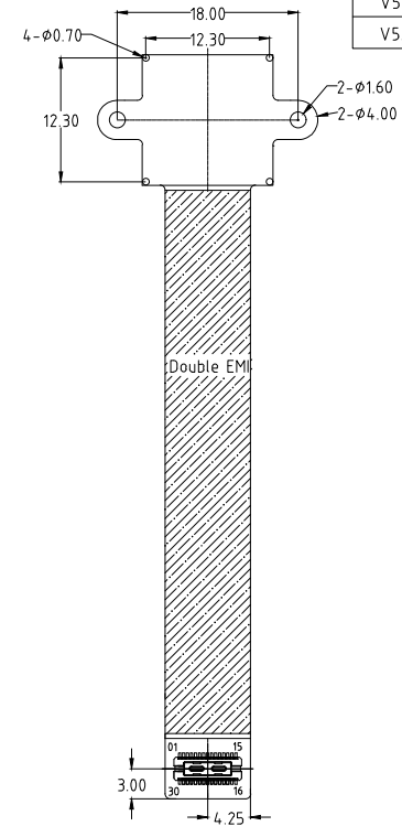
BOTTOM VIEW
